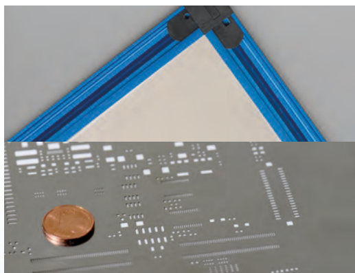
SMD Stencils
